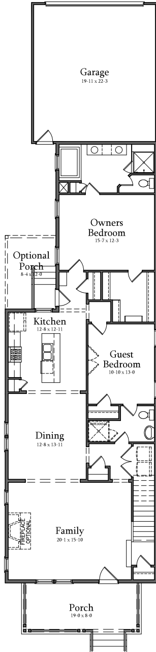
Opt. First Floor Plan
