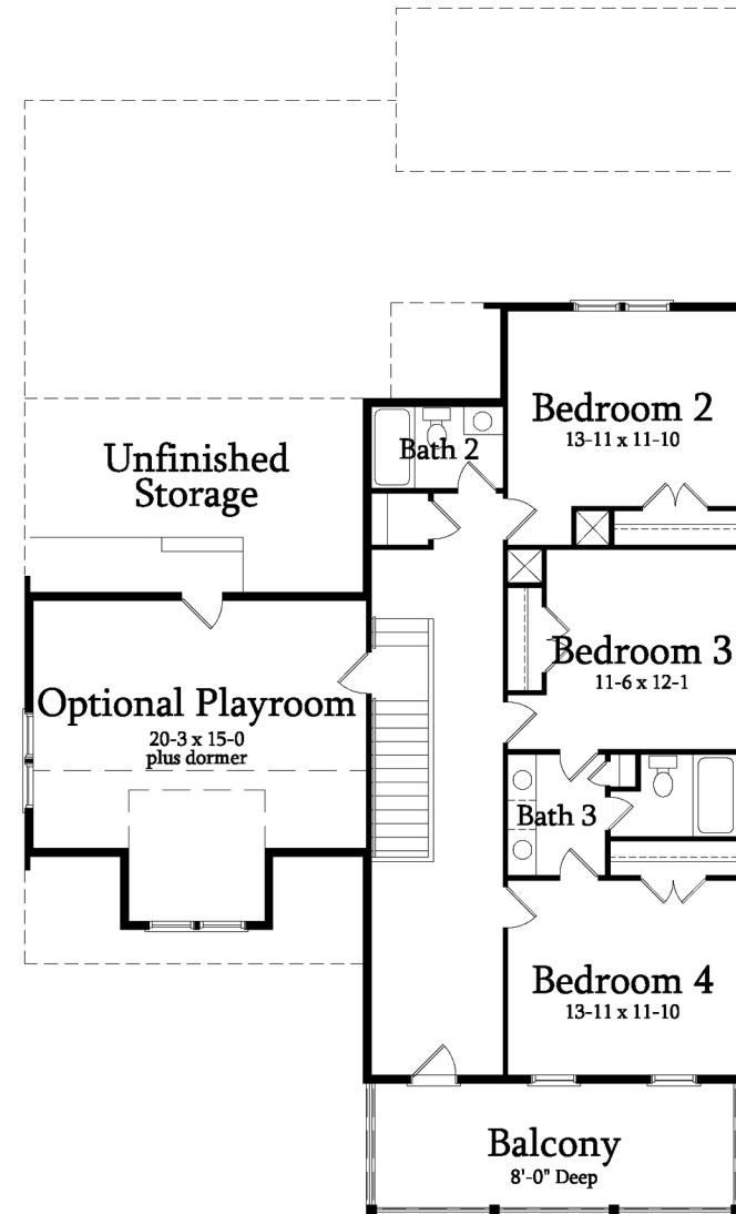
Second Floor
