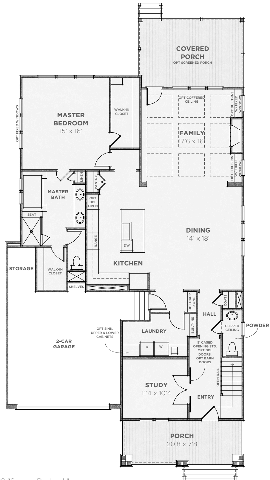
FIRST FLOOR
