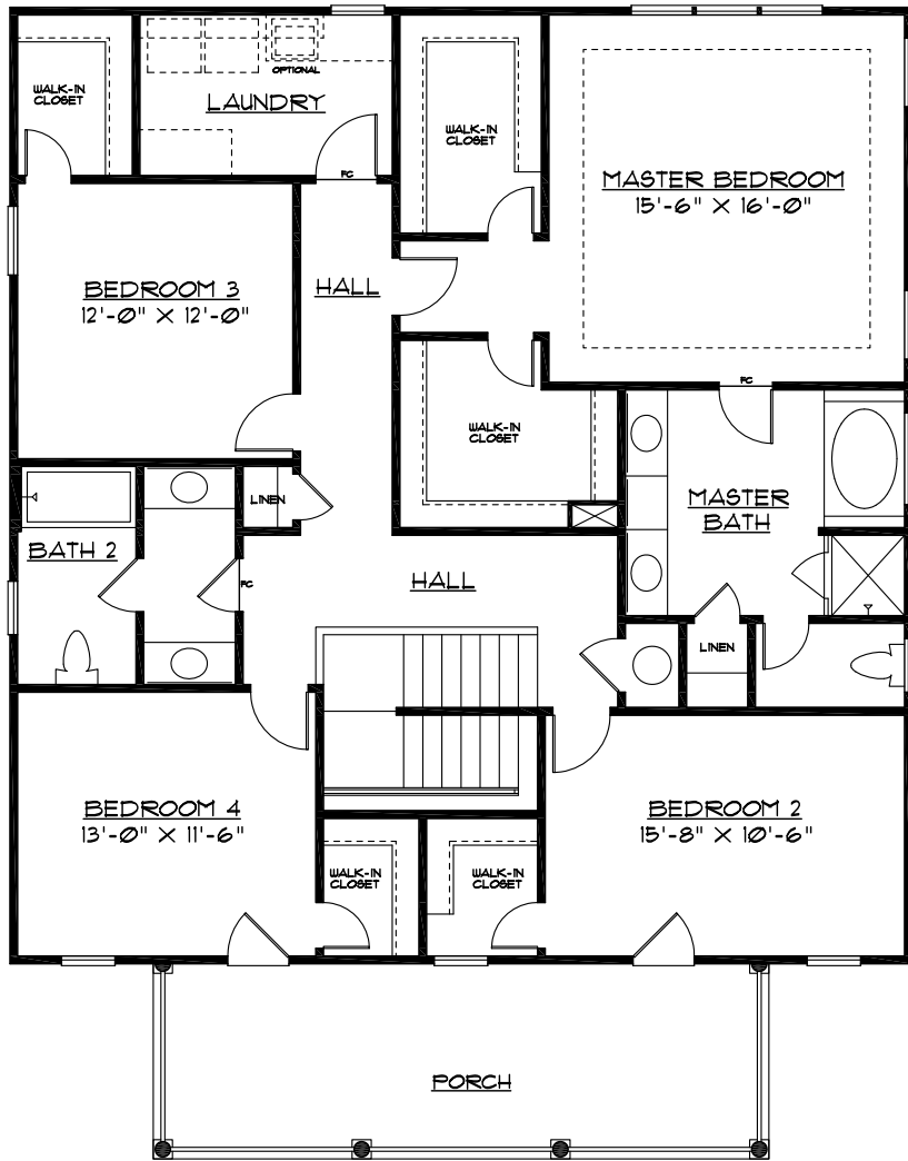
SECOND FLOOR PLAN HAMPTON - B
