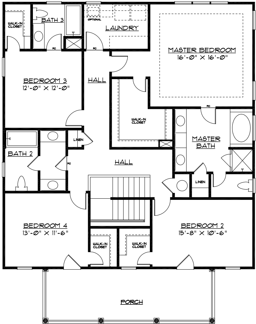
ALT. SECOND FLOOR PLAN HAMPTON - B
