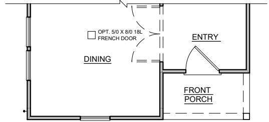
FIRST FLOOR PLAN 1/4" = 1'-0" 2245 F
