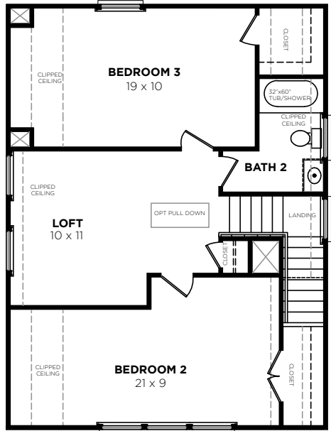
SECOND FLOOR 2098-P BARRINGTON 4/13/23
