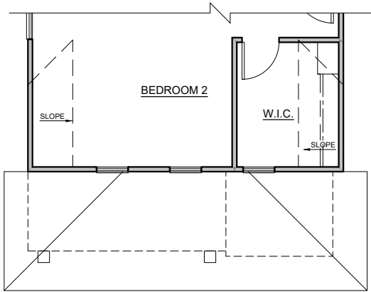
SECOND FLOOR PLAN 1/4" = 1'-0" 2275 F
