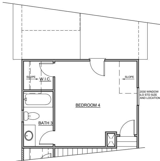
OPT. BEDROOM 4 (+219 SQ.FT) BATH 3 (+54 SQ.FT) WITH WALK IN CLOSET
