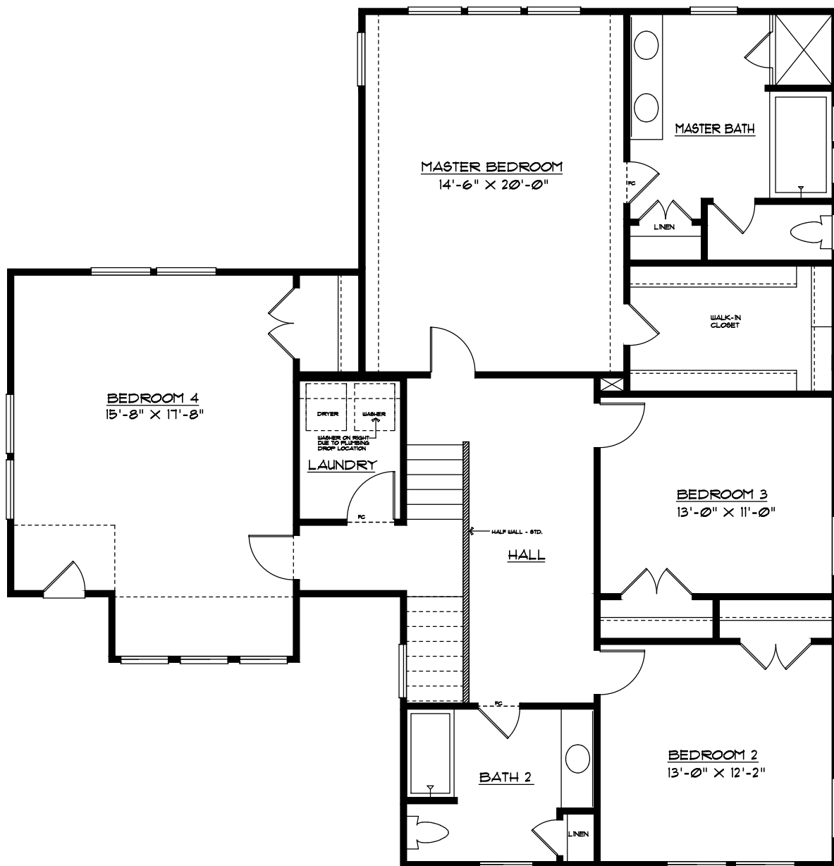
SECOND FLOOR PLAN BERKELEY - D/G
