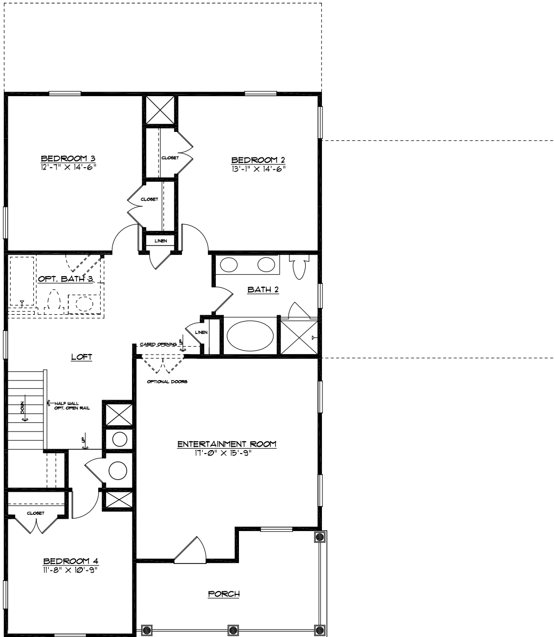
ALTERNATE SECOND FLOOR PLAN BRITTANY-F/G
