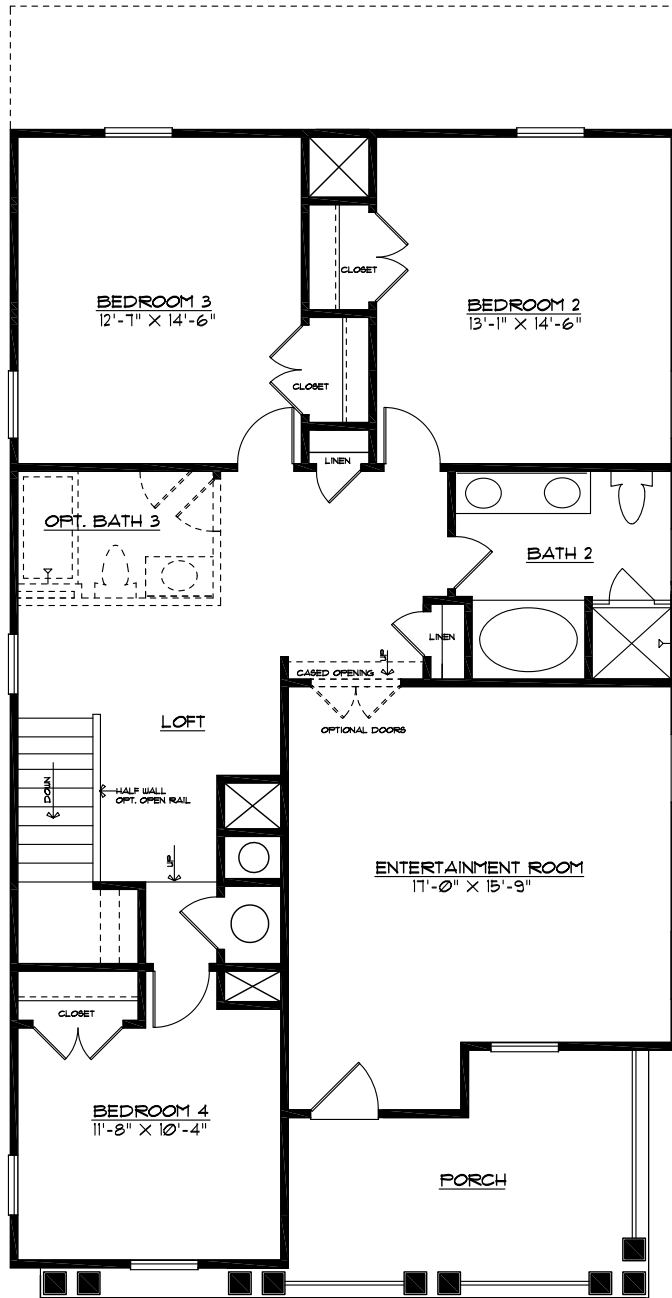
ALTERNATE SECOND FLOOR PLAN BRITTANY-D
