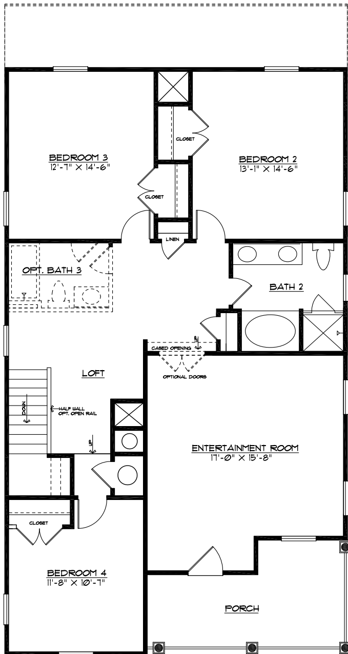
ALTERNATE SECOND FLOOR PLAN BRITTANY -F
