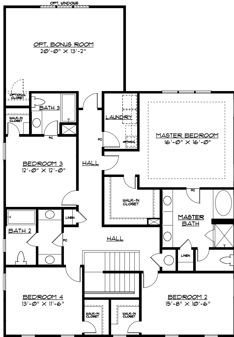
ALT. SECOND FLOOR PLAN HAMPTON - C/G
