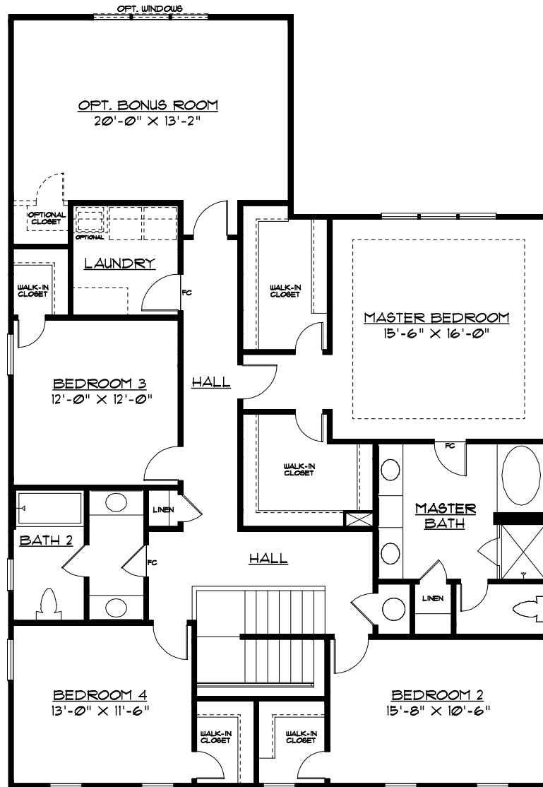
SECOND FLOOR PLAN HAMPTON - C/G
