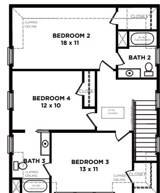
OPT SECOND FLOOR PLAN W/ BEDROOM 4 AND BATH 3
