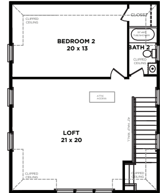
STANDARD SECOND FLOOR PLAN
