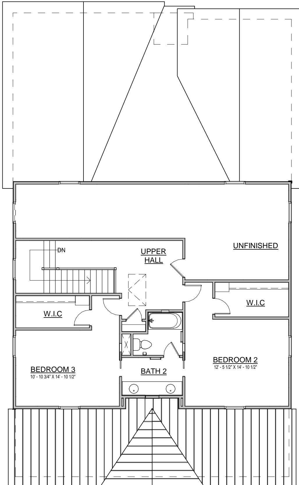
SECOND FLOOR PLAN HEATED (862 SQ. FT.) UNFINISHED (409 SQ. FT.)
