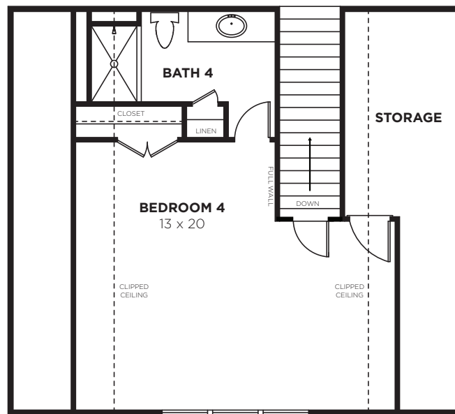
LAUREL 2555A SECOND FLOOR BEDROOM 4 & BATH 4 (OPTIONAL)
