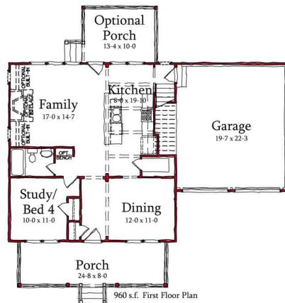
Optional First Floor Plan
