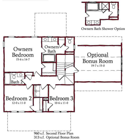
Optional Second Floor Plan
