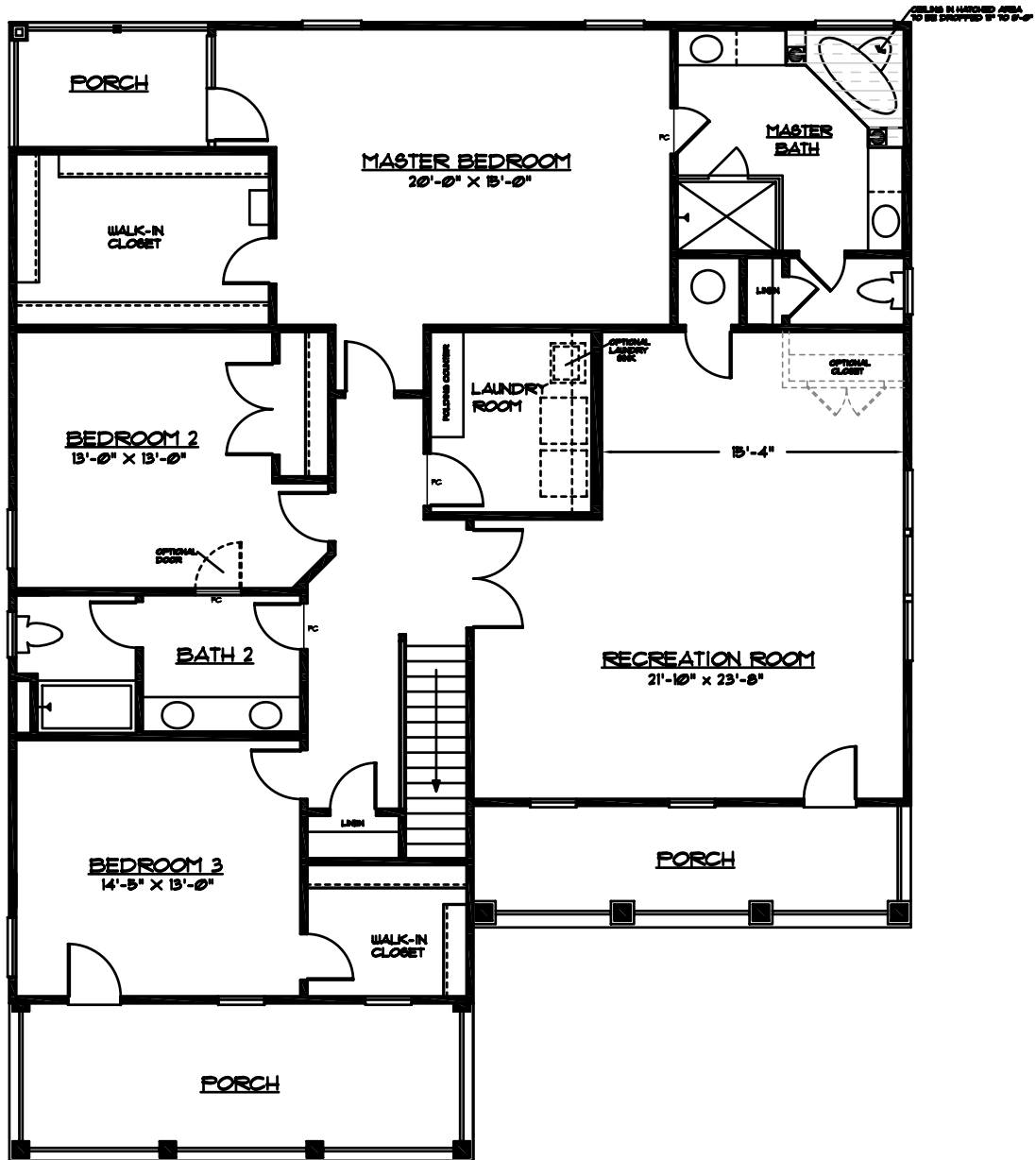
SECOND FLOOR PLAN RIDGE - A
