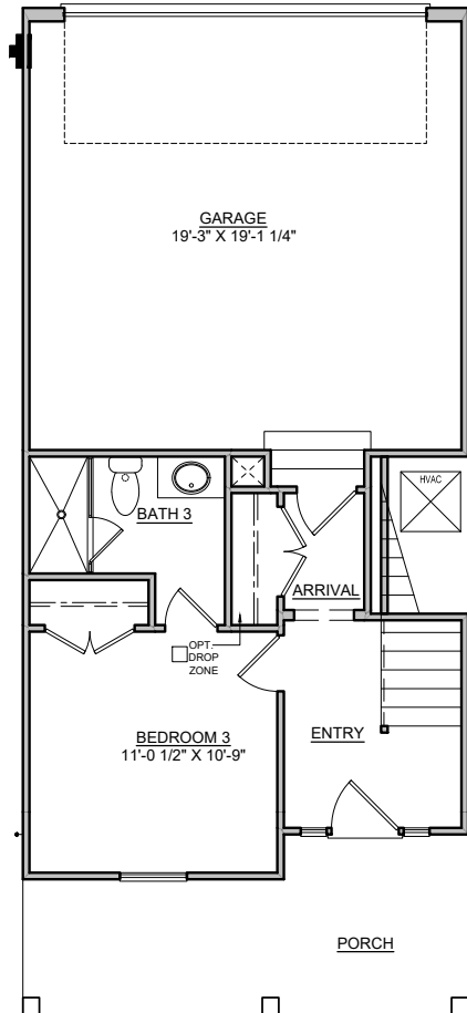
FIRST FLOOR PLAN 1/4" = 1'-0" 1829 L
