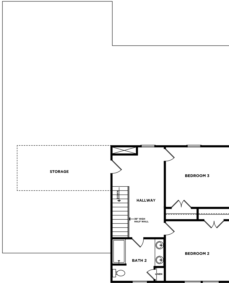
RUTLEDGE-A SECOND FLOOR PLAN
