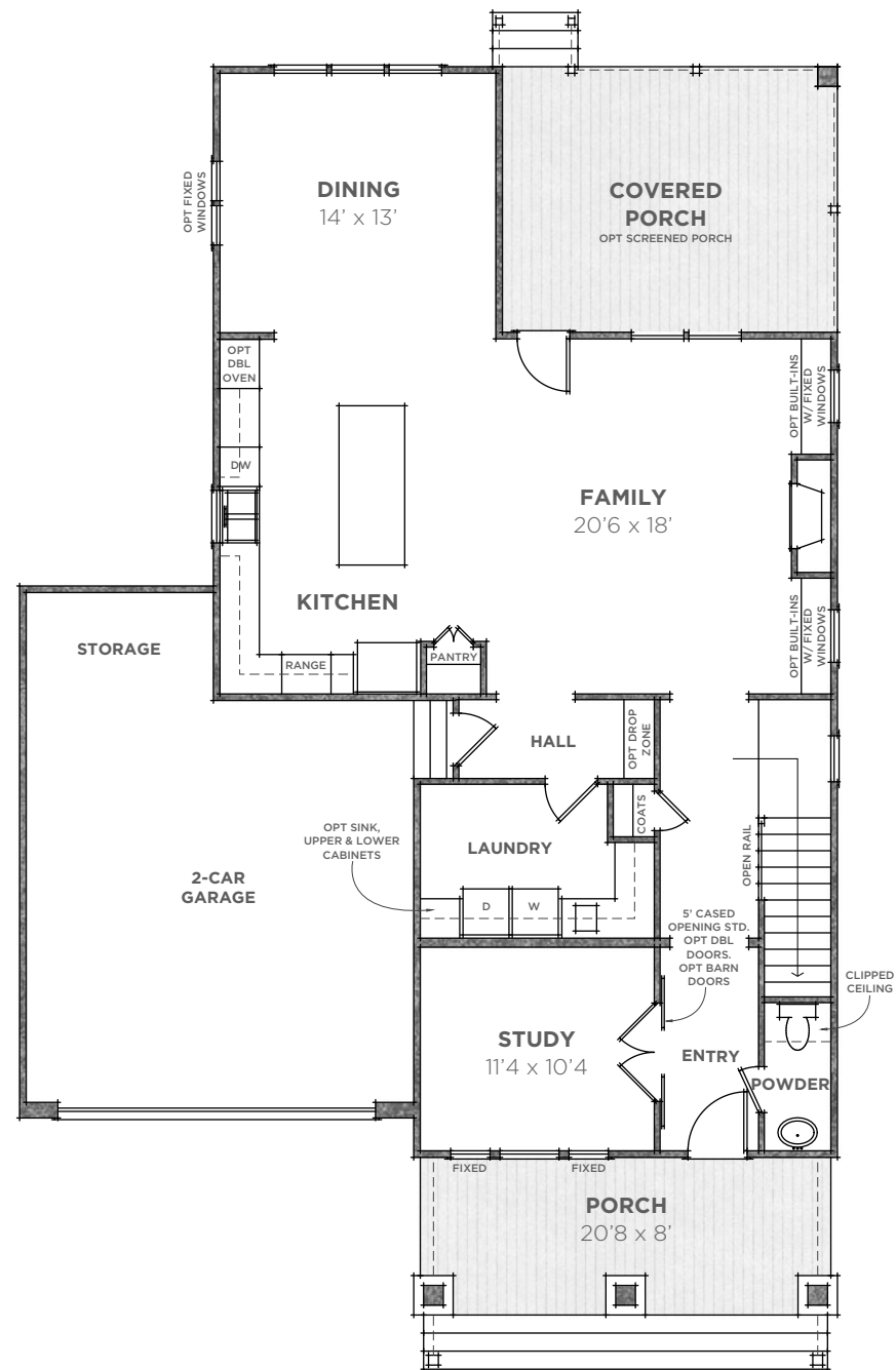
FIRST FLOOR
