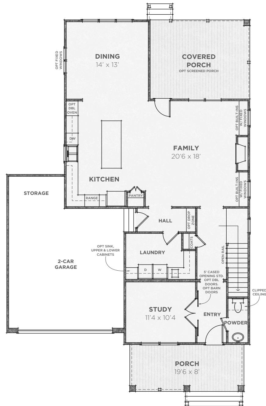
FIRST FLOOR
