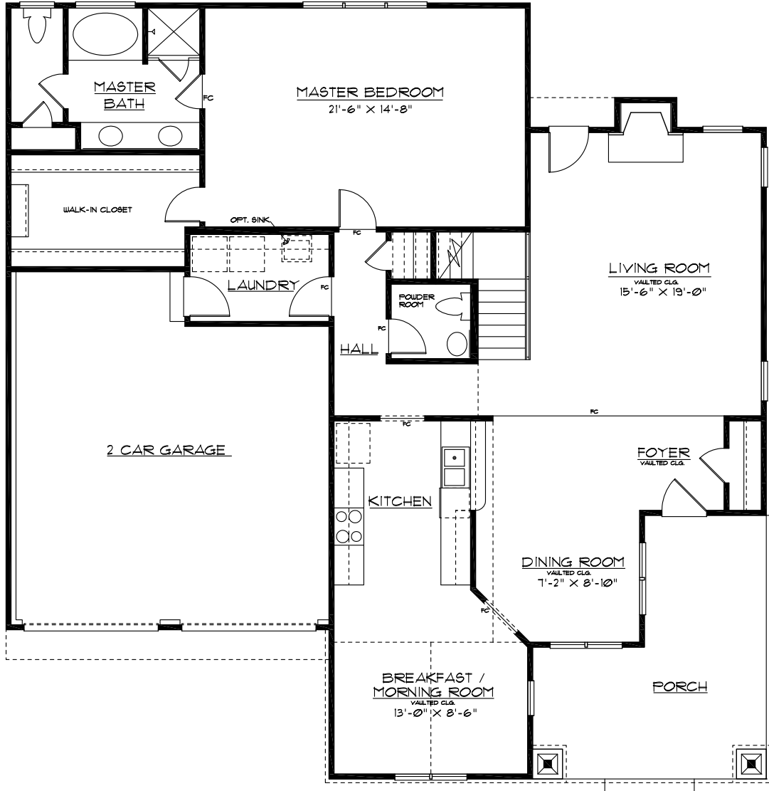
FIRST FLOOR PLAN TYLER - N
