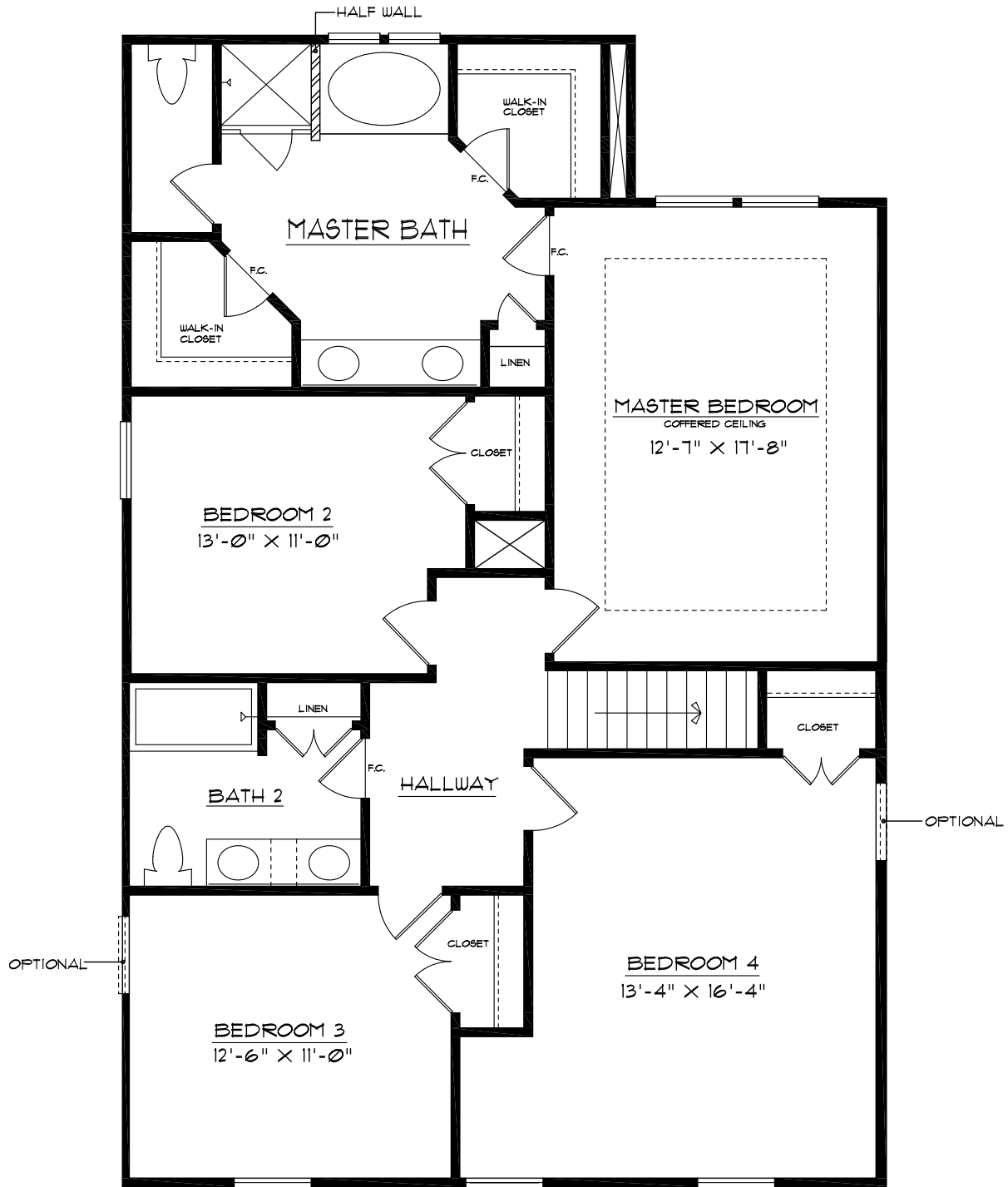
SECOND FLOOR PLAN WENDOOVER - A
