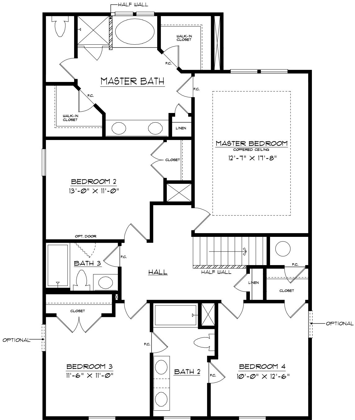
ALTERNATE SECOND FLOOR PLAN WENDOVER - C
