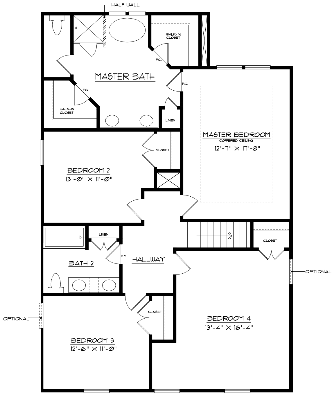
SECOND FLOOR PLAN WENDOVER - C
