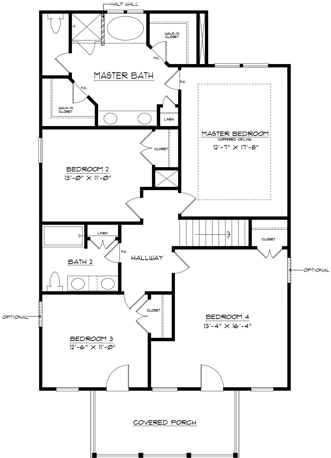
SECOND FLOOR PLAN WENDOVER - D
