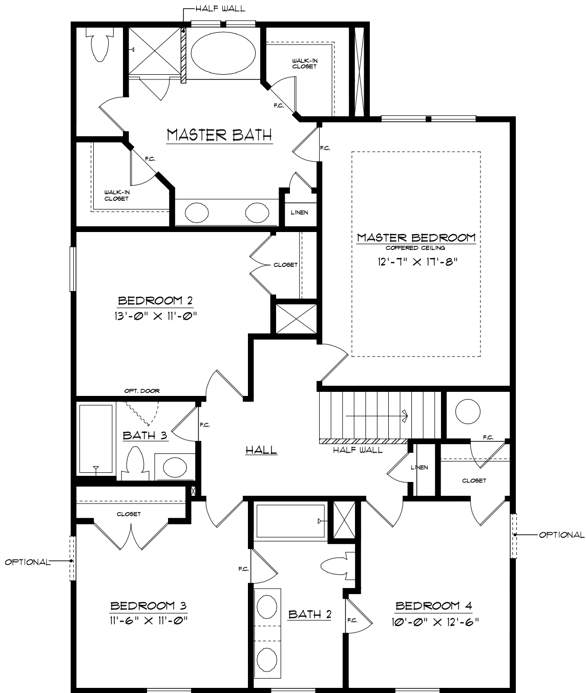
ALTERNATE SECOND FLOOR PLAN WENDOVER - E
