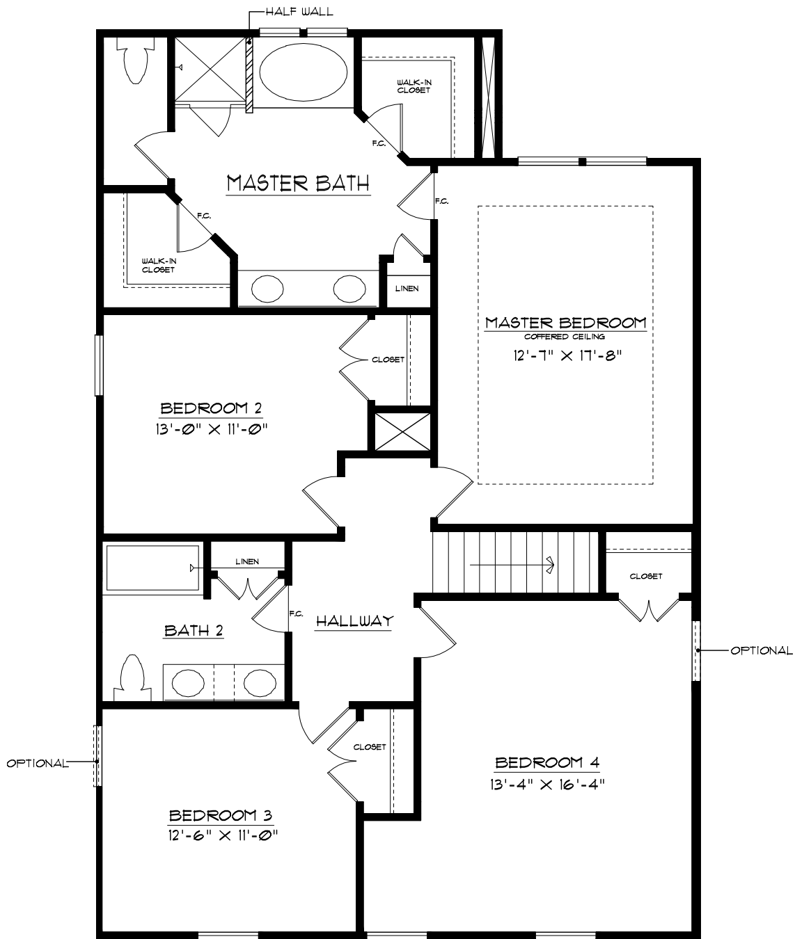
SECOND FLOOR PLAN WENDOVER - E
