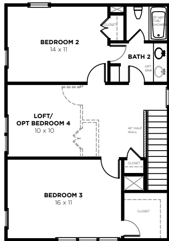
SECOND FLOOR 2264G- WINSLOW 3/1/24
