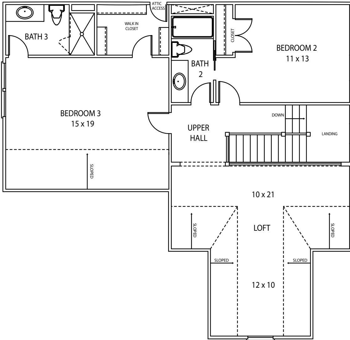
UPPER LEVEL 3526B
