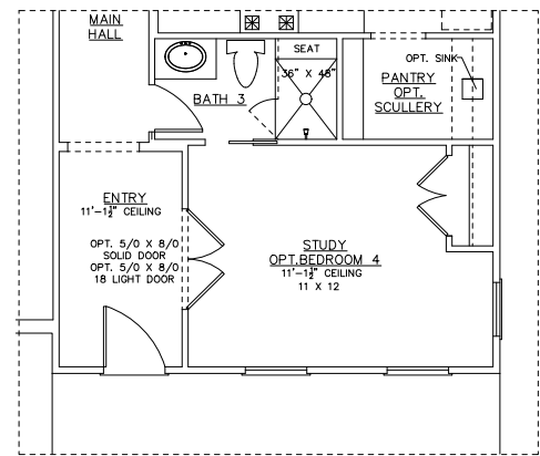
OPT SCULLERY LAYOUT "B" WITH BEDROOM 4 / BATH 3
