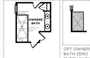
OPT EXPANDED OWNERS' SHOWER LAYOUT
