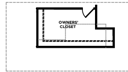
OPT EXPANDED OWNERS' CLOSET (AVAIL. ON STD. LAYOUT ONLY)
